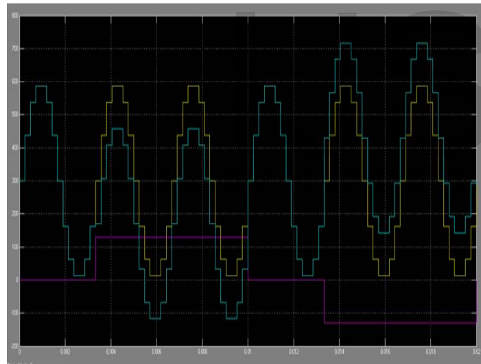
Fig. 2(a): Mixing seven-level, six-pulse signals, and transformer's ratios to attain V_{YU} and V_{\Delta U}
