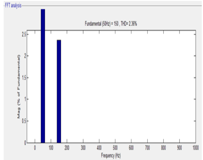
Fig. 2(b): Harmonic content
