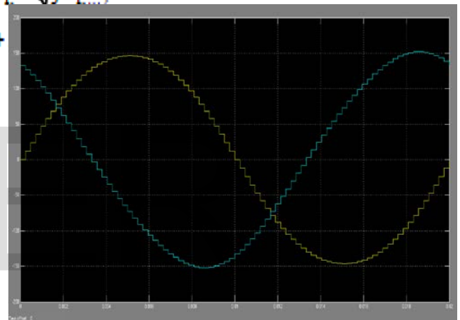
Fig. 3: 12-pulse seven level 3 phase output voltage
