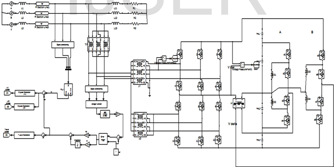
Fig.1: Twelve pulse seven level STATCOM structure
